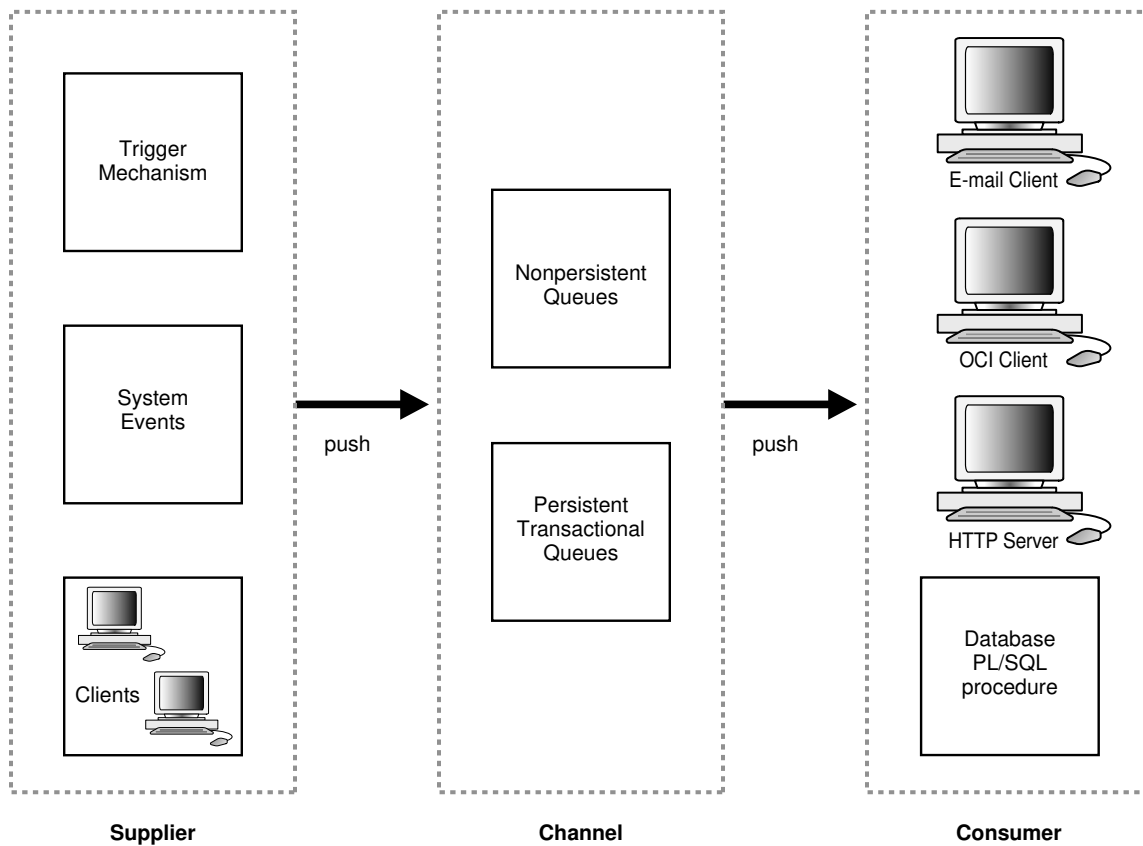
Figure 12-1 Publish-Subscribe Model
