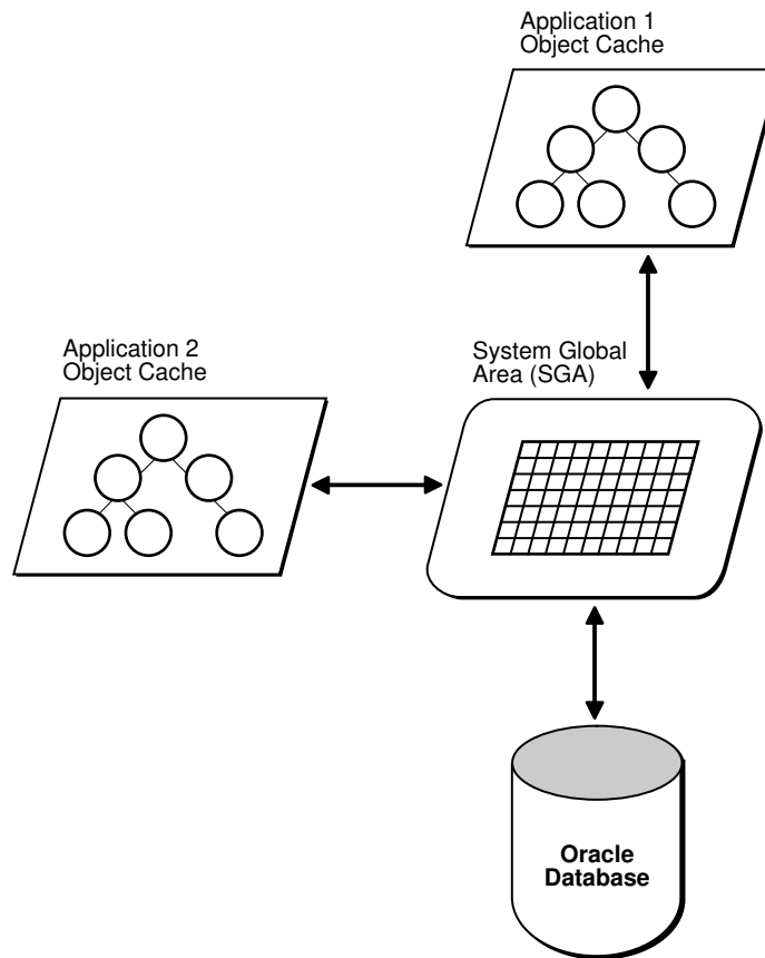
Figure 21-1 Object Cache
